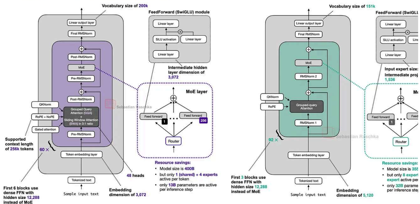
Figure 54: Arcee AI Trinity Large next to GLM 4.5 of a relatively similar size (400B vs 355B).
